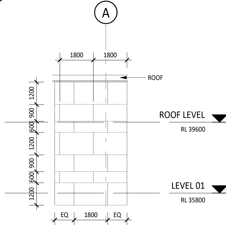
4 BUILDING ELEVATION - TYPICAL CFC PATTERN 30-11 1 : 100
