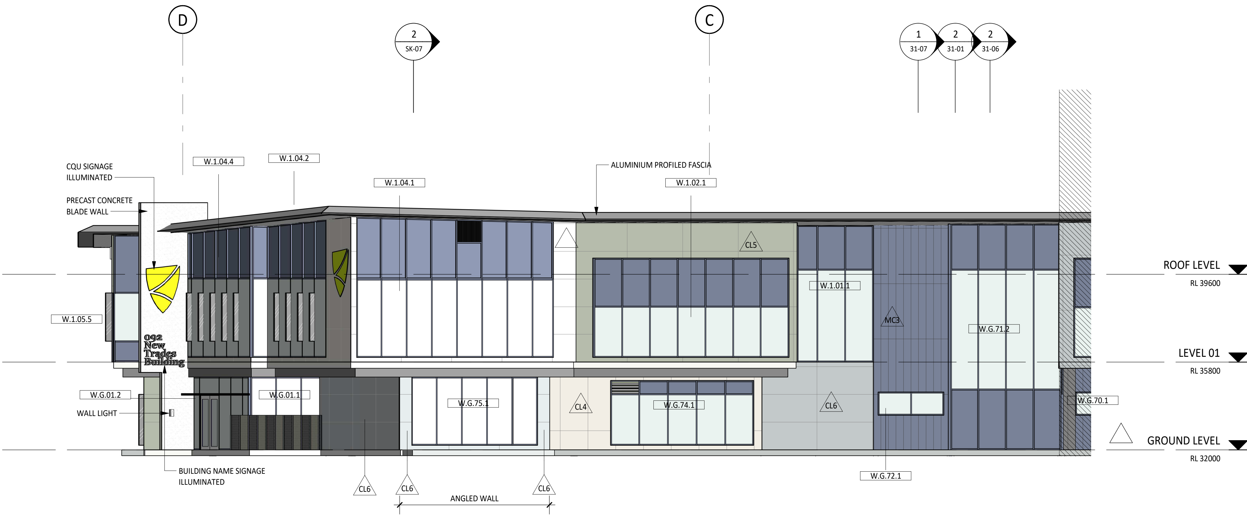
1 BUILDING ELEVATION - SOUTH - 1 21-00 1 : 100
