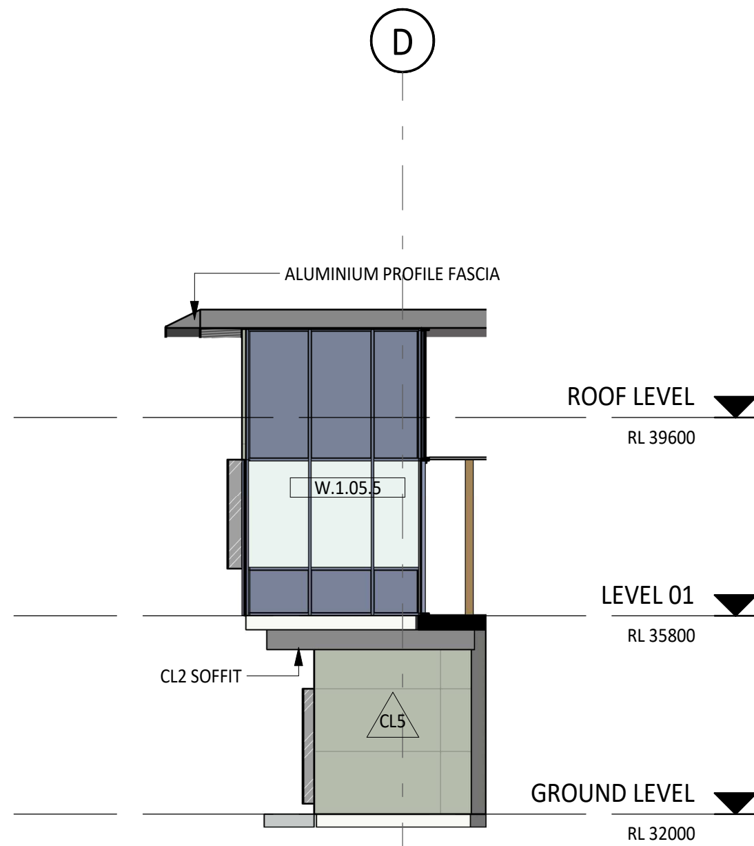
3 BUILDING ELEVATION - SOUTH - 3 21-00 1 : 100
