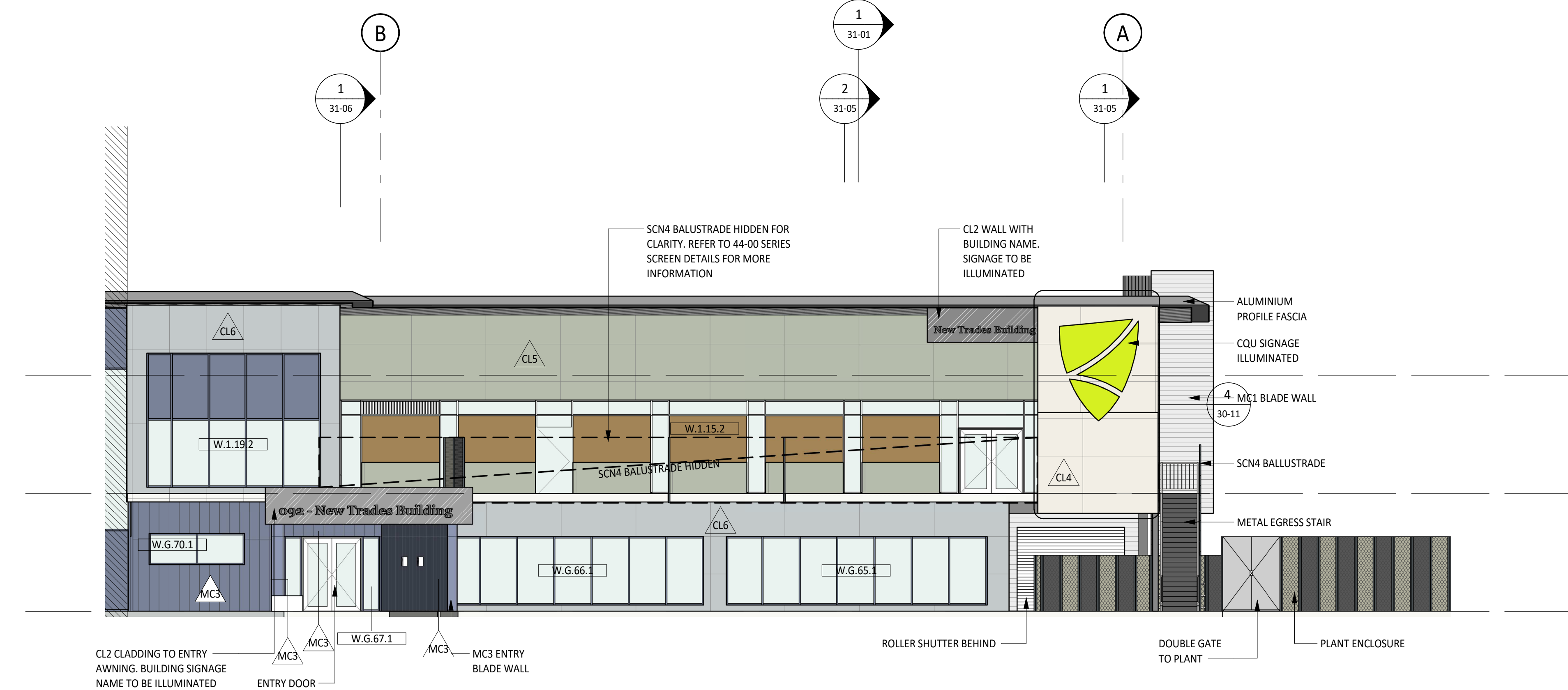
1 BUILDING ELEVATION - SOUTH - 1 21-00 1 : 100
